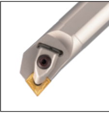
DCLN□95°
