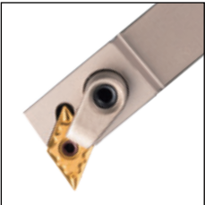
MDUN□95°
